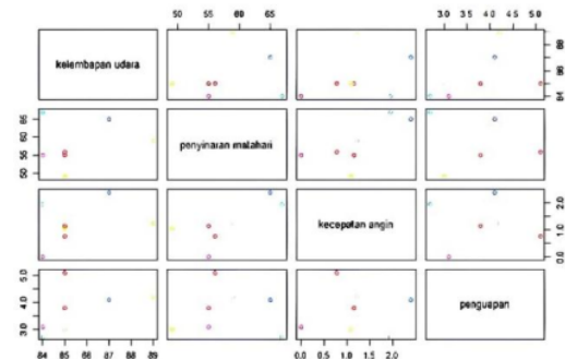
Gambar 3. Pair Plot
