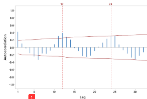
Gambar 5. Plot ACF Curah Hujan
