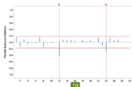
Gambar 7. Plot PACF
