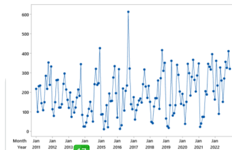
Gambar 2. Time Series Plot Curah Hujan
