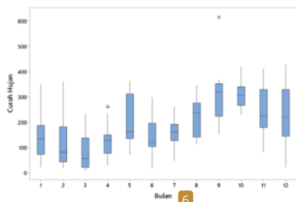
Gambar 3. Box Plot Curah Hujan
