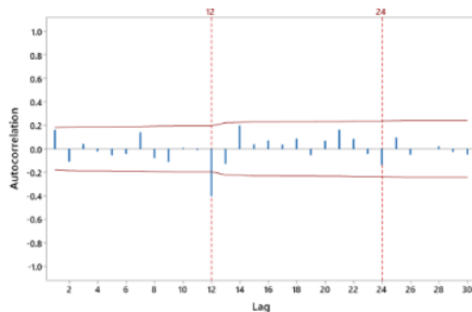
Gambar 6. Plot ACF Differencing
