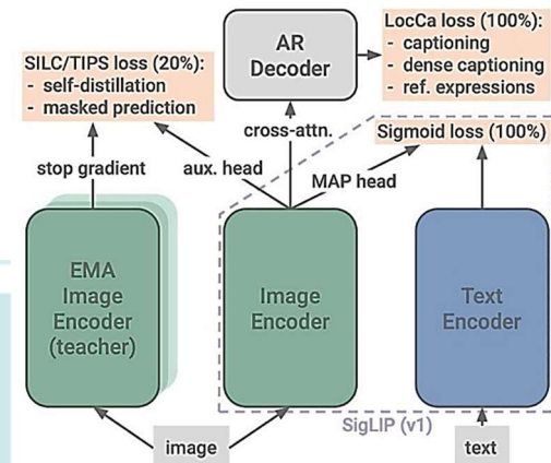
Figure 4. SigLIP 2 training recipe using sigmoid-based contrastive loss (Tschannen et al., 2025). This study uses the So400m variant at 384×384 resolution.
