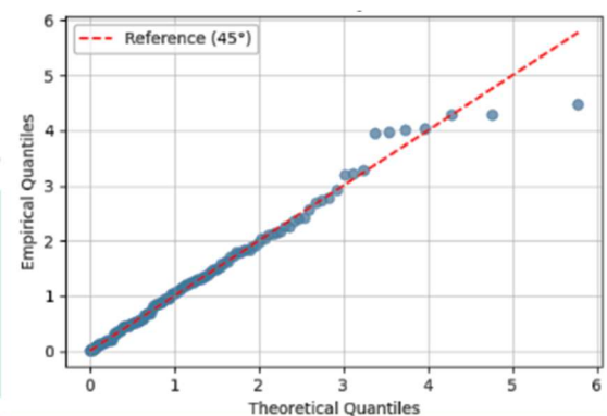
Figure 6. Q-Q Plot of MGRD
