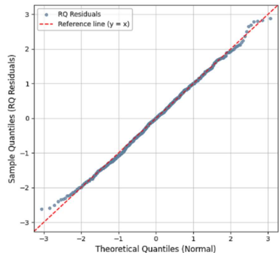
Figure 3. Q-Q Plot of ZIPL
