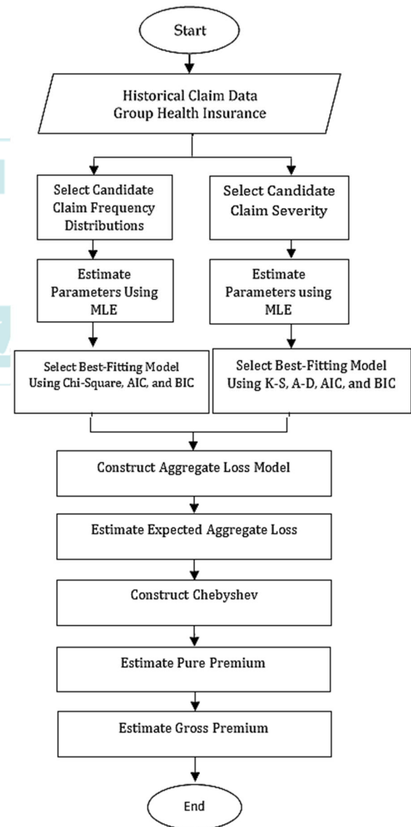
Figure 1. Research Workflow
