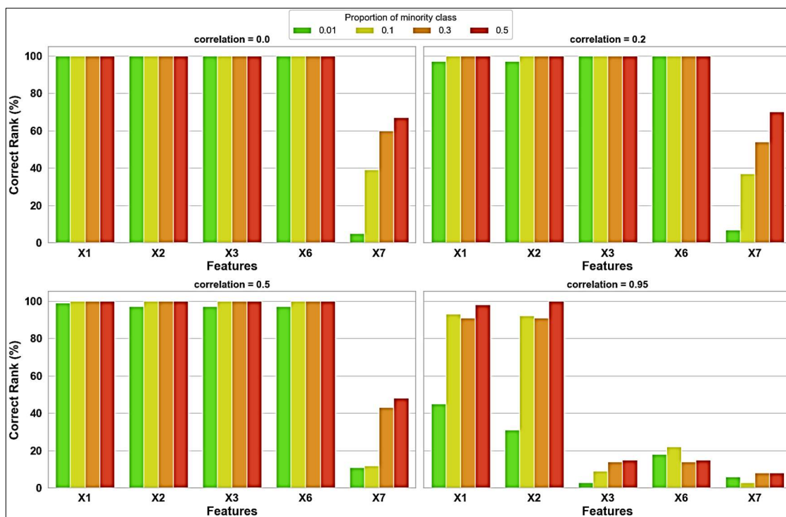
Figure 4. Percentage of correct feature ranking for X_1 , X_2 , X_3 , X_6 , and X_7 across 100 repetitions of the LightGBM model under different correlation levels in number of features 15.
