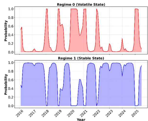
Figure 3. Smoothed Marginal Probability Plot Data
